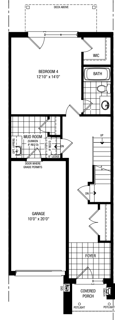
PARTIAL OPT. GROUND B 4 BEDROOM PLAN
