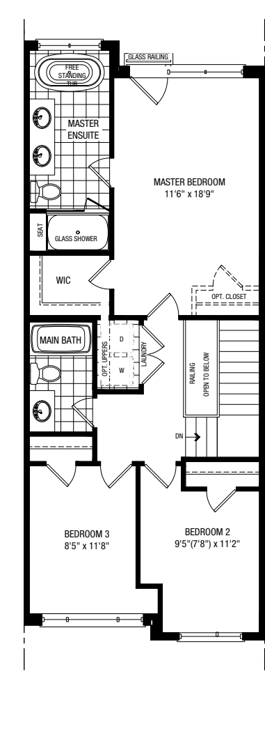
PARTIAL THIRD B
