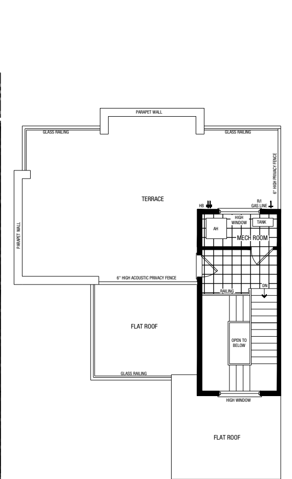
TERRACE A BLOCK 5 UNIT 27 & BLOCK 14 UNIT 80
