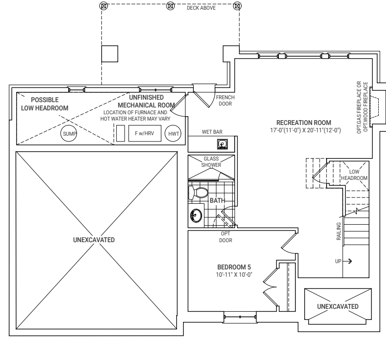
OPT. FINISHED BASEMENT PLAN ELEVATION A
