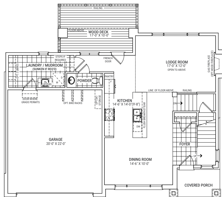
GROUND FLOOR PLAN ELEVATION B
