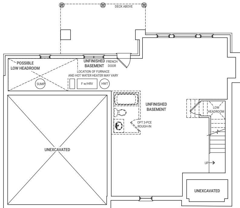
BASEMENT PLAN ELEVATION A
