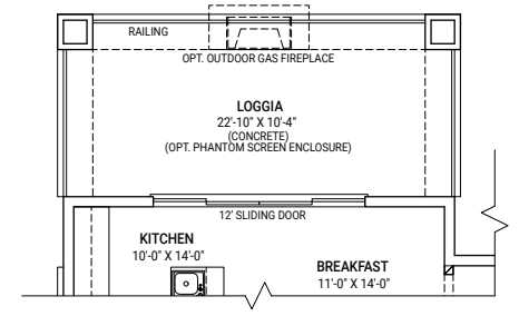
PARTIAL GROUND FLOOR PLAN W/ OPT. LOGGIA
