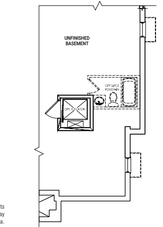
PARTIAL BASEMENT PLAN ELEVATION A & D W/ OPT. ELEVATOR
