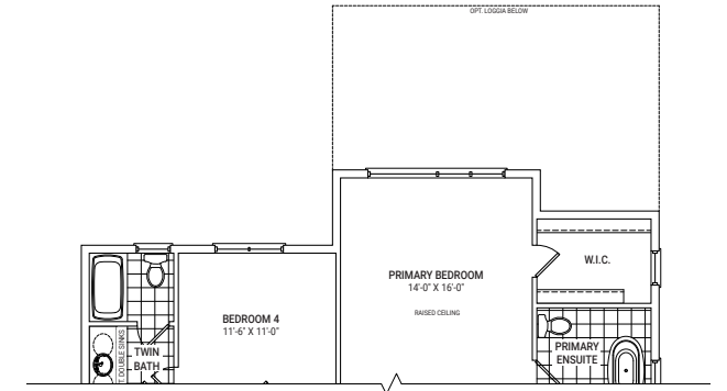
PARTIAL SECOND FLOOR PLAN ELEVATION A W/ OPT. LOGGIA
