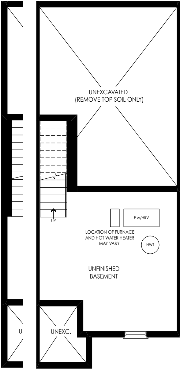
END BASEMENT ELEV. C ELEV. C
