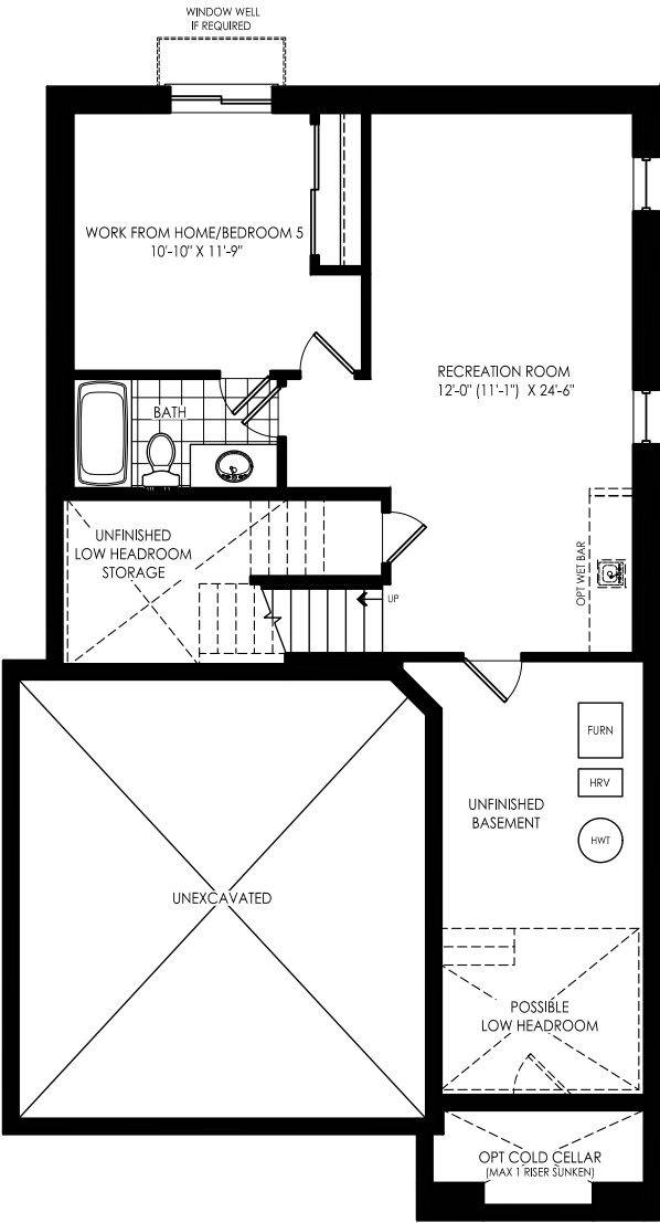
OPT. FINISHED BASEMENT ADDS 614 SQ.FT. ELEV. A
