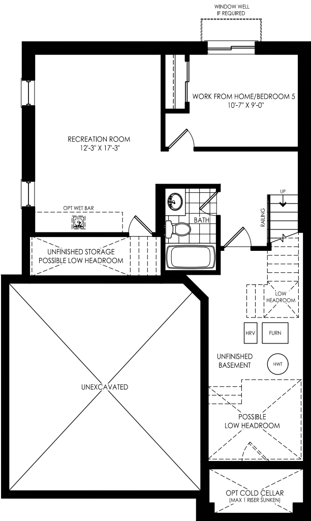
OPT. FINISHED BASEMENT ADDS 531 SQ.FT. ELEV. A
