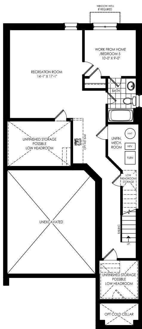
OPT. FINISHED BASEMENT ADDS 681 SQ.FT ELEV. A
