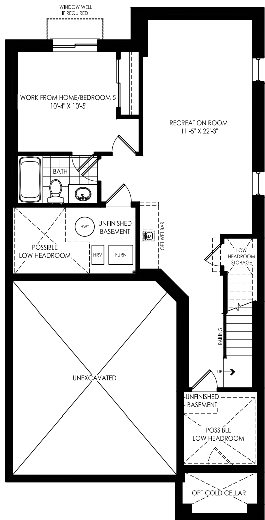
OPT. FINISHED BASEMENT ADDS 650 SQ.FT. ELEV. A
