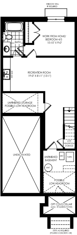
OPT. FINISHED BASEMENT ELEV. A & B & C
